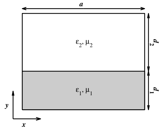
Fig. 10. Partially filled waveguide [8].
