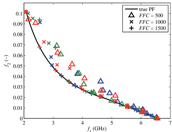
Fig. 14. Elements of the non-dominated sets computed by MOPSO (blue), NSGA-II (green) and MOSOMA (red) after 500, 1 000 and 1 500 evaluations of the objective function.
